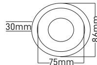
URSA SIVA ALTI MODERN DEKORATİF MX-2019 SPOT
